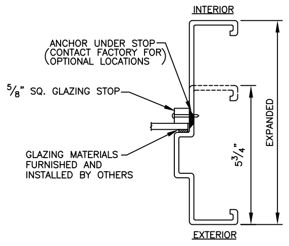
GLAZING PLACEMENT
