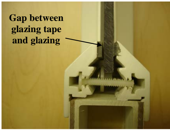
Incorrect Installation
